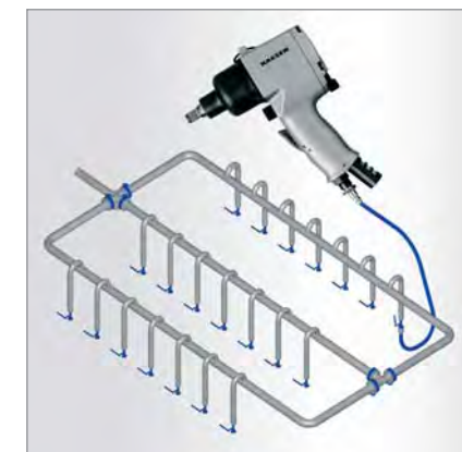
Fig. 4: Leakage measurement of compressed air consumers + air distribution network
