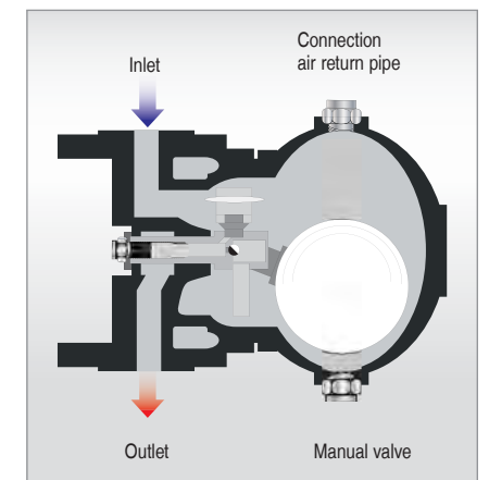
Fig. 4: Float drain for compressed air condensate
