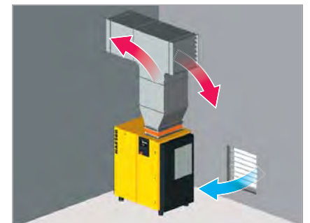
Fig. 4: A thermostatically-controlled flap directs warm air into the compressor room in winter
