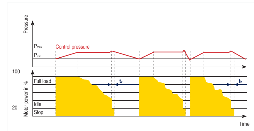
Fig. 5: Continuous delivery control via motor speed (frequency conversion)
