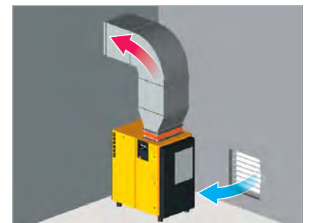
Fig. 3: Forced ventilation with exhaust ducting for machines above 11 kW
