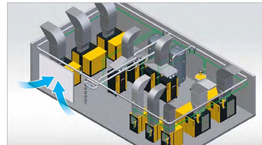
Fig. 2: Compressed air station with supply air system
