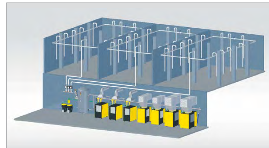
Fig. 4: Compressed air supply with a central compressed air station for multiple production areas
