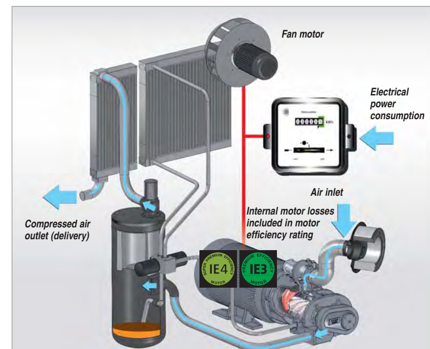
Fig. 2: Basic layout of a rotary screw compressor; determining specific power
