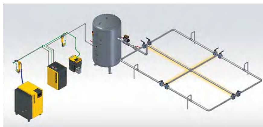
Fig. 2: Expansion of distribution pipework capacity using cross-connection lines
