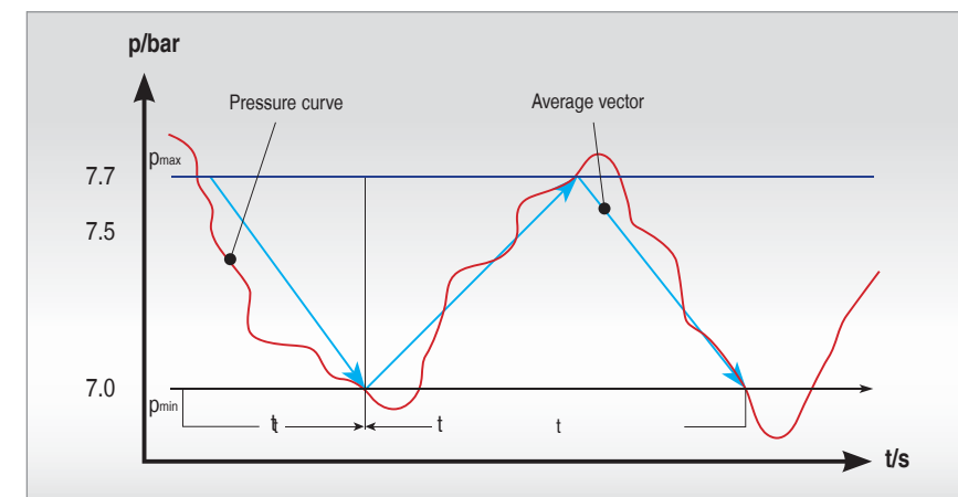
Fig. 2: Optimum pressure is set taking all control-relevant losses into account
