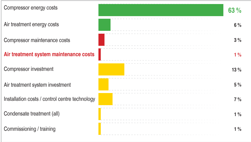
Fig. 2: The cost structure of an optimised compressed air system
