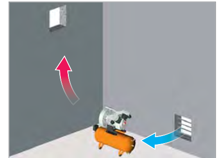
Fig. 1: Natural ventilation for compressors up to 5.5 kW
