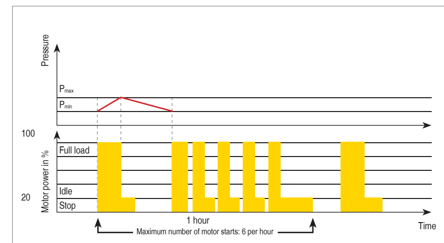
Fig. 4: Vario control with variable calculated idling periods
