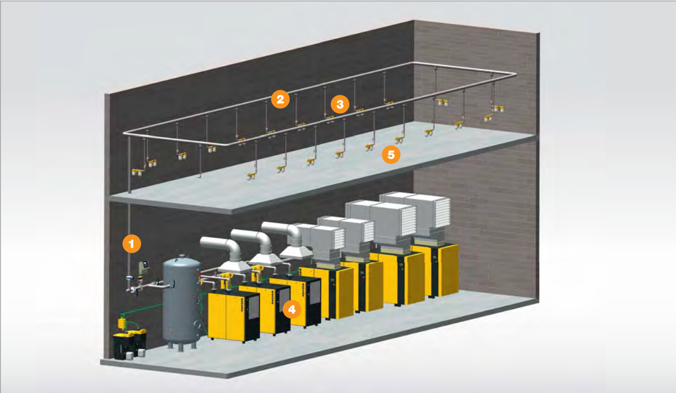
Fig. 1: Main components of a compressed air distribution system: Air-main (1), Distribution piping (2), Connection piping (3), Dryer (4), Maintenance unit/hose (5)
