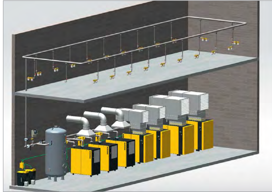
Example of a compressed air station with exhaust air system and thermostatically controlled additional ventilation for the refrigeration dryers
