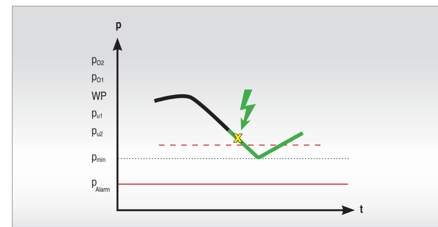
Fig. 4: The system prevents undershooting of the preset minimum demand pressure
