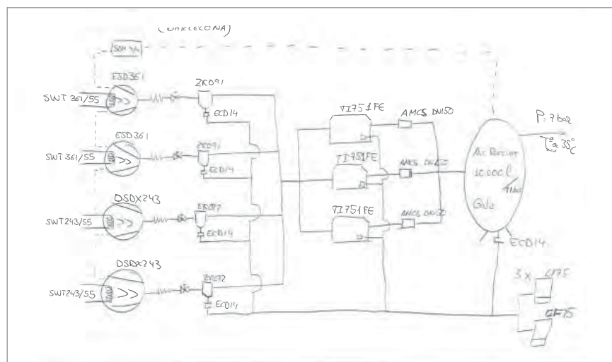
Fig. 4: Hand-drawn P & I diagram of a compressed air station
