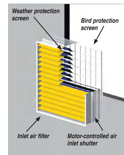
Fig. 1: Supply air system (design)
