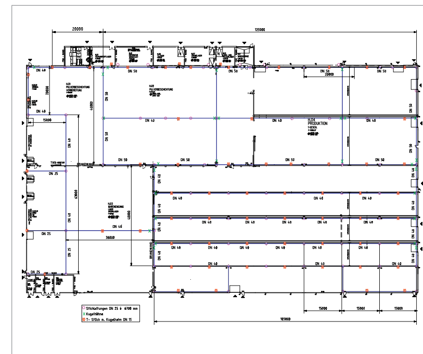
Fig. 3: Layout of a compressed air distribution network
