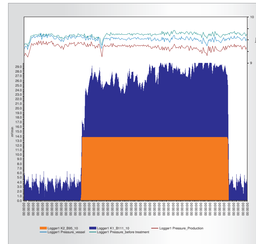
Fig. 8: A business's pressure and compressed air consuming structure measured with ADA.
