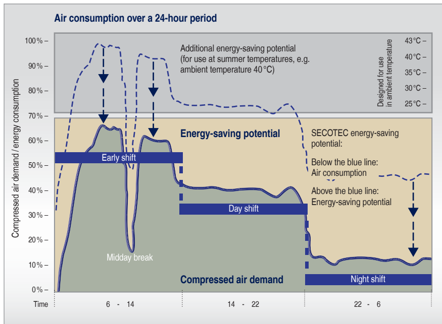
Fig. 3: Energy-saving potential of refrigeration dryers with cycling control
