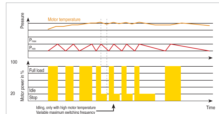
Fig. 3: Dynamic control, based on Dual control, with drive motor temperature dependent idling
